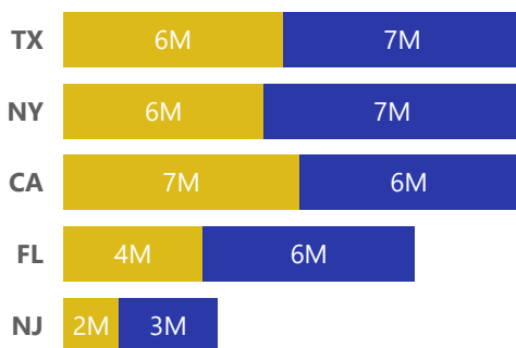
Top 5 States
